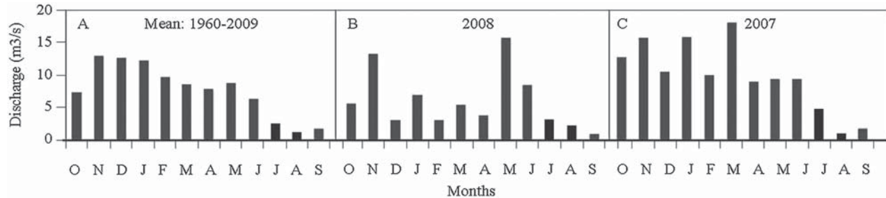
Figure 2. Tsable River water-year hydrographs. Dark bars indicate the reconstruction season (July–August). (A) Gauged mean monthly discharge over the length of record used (1960–2009); (B) mean monthly discharge in a ‘more nival’ year when runoff during spring snowmelt outweighed rain-derived runoff during winter; (C) mean monthly discharge in a ‘more pluvial’ year when runoff from winter rains outweighed runoff from spring snowmelt
